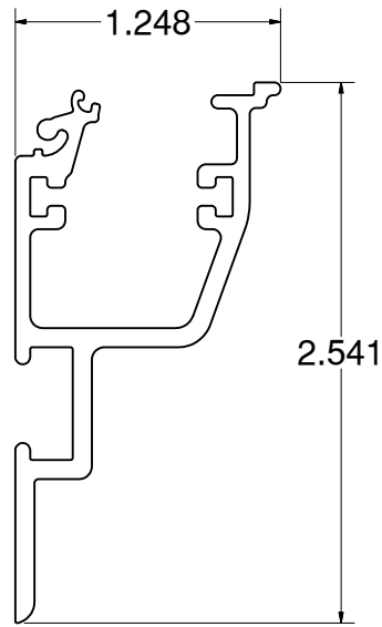
Soft Signage Narrow Snap Tension Frame Part# 3091N
